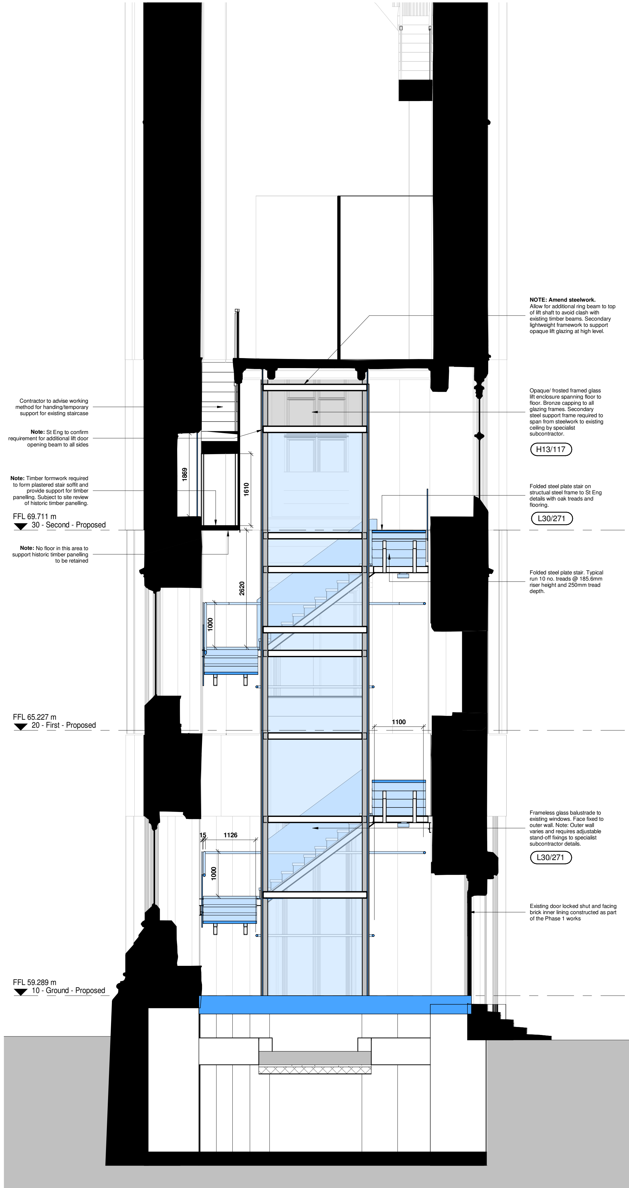
2D View 1 : 50
