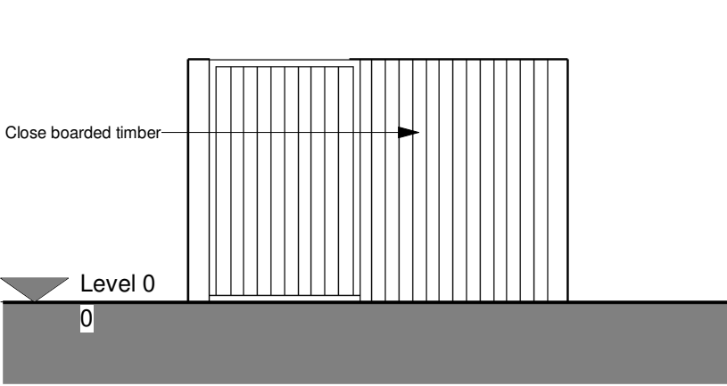
North Elevation_Bin Store 01 1 : 50
