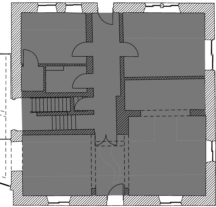
farmhouse ground floor 111.59 m 2
