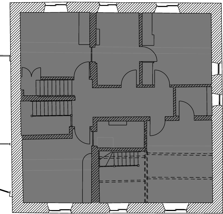
farmhouse first floor 112.84 m 2
