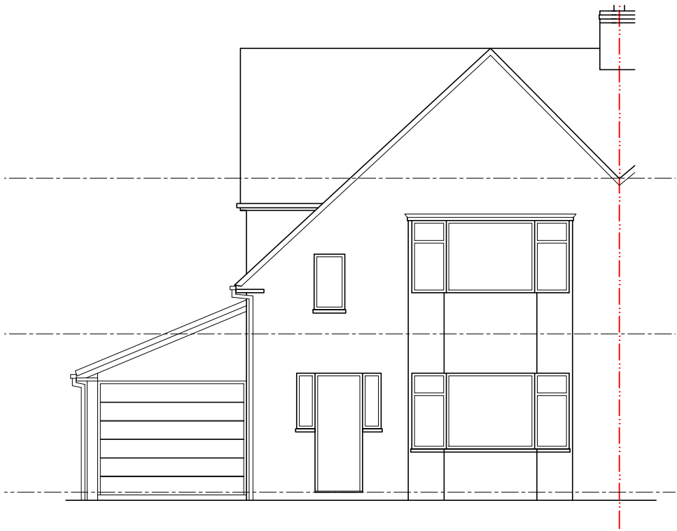
North Facing Front Elevation
