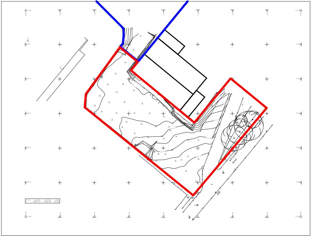
2 Existing Location Plan 1 : 1250
