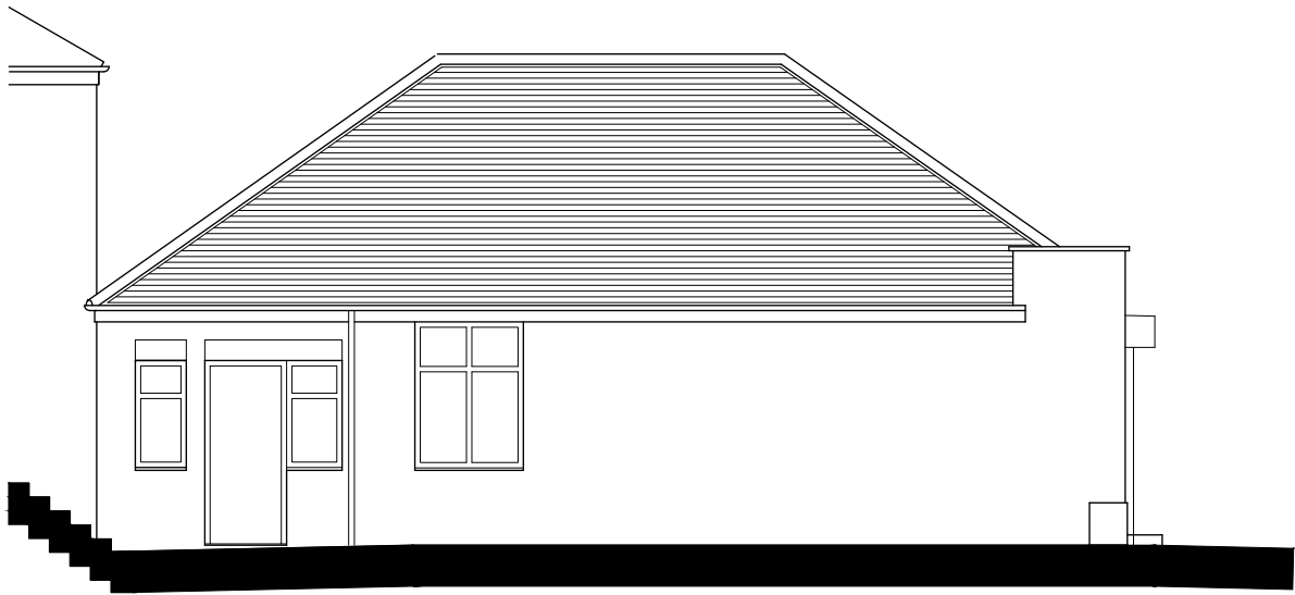
Side Elevation to 213 Manchester New Road as Proposed
