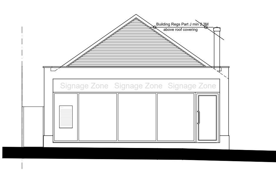
Elevation to Manchester New Road as Proposed
