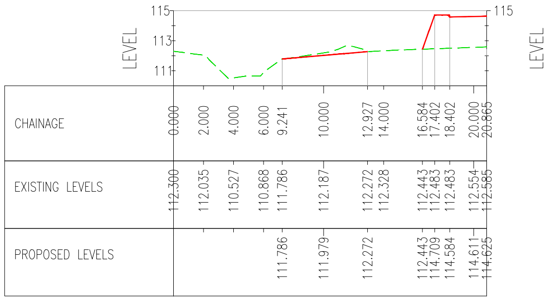
SECTION L-L
