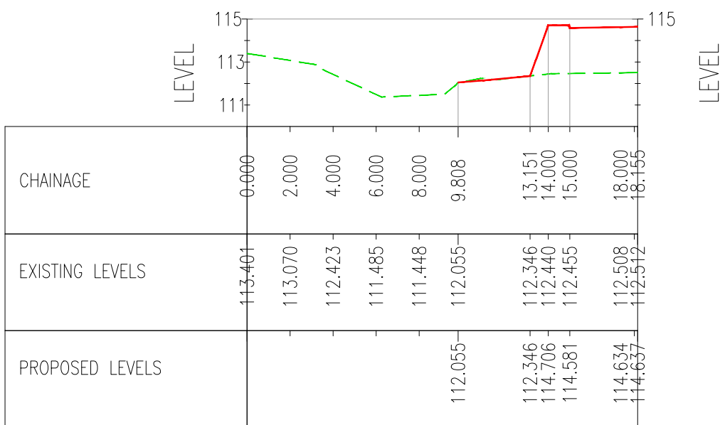
SECTION N-N
