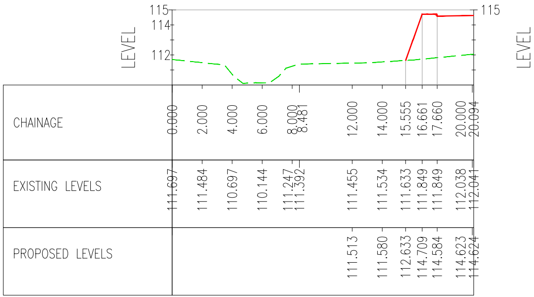
SECTION K-K
