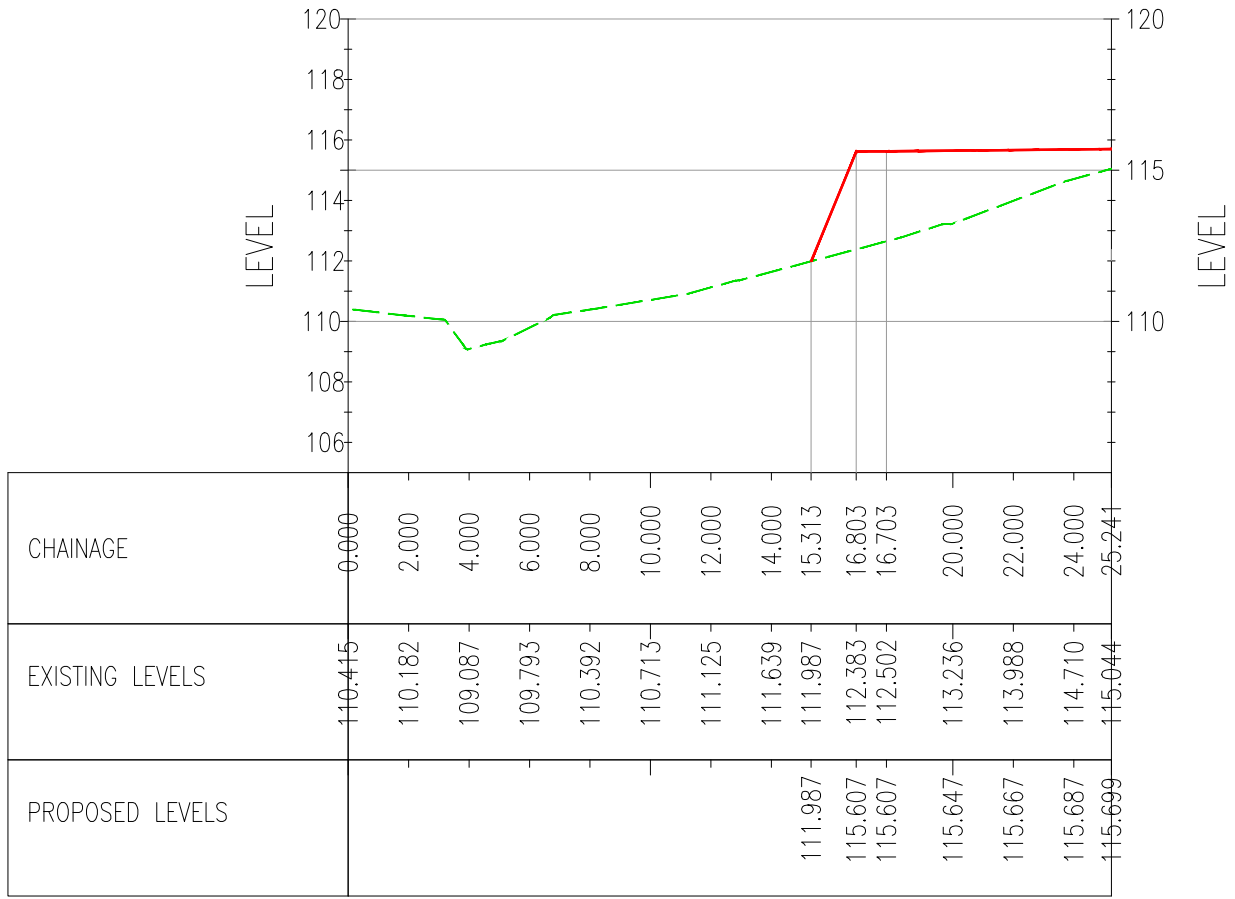
SECTION P-P
