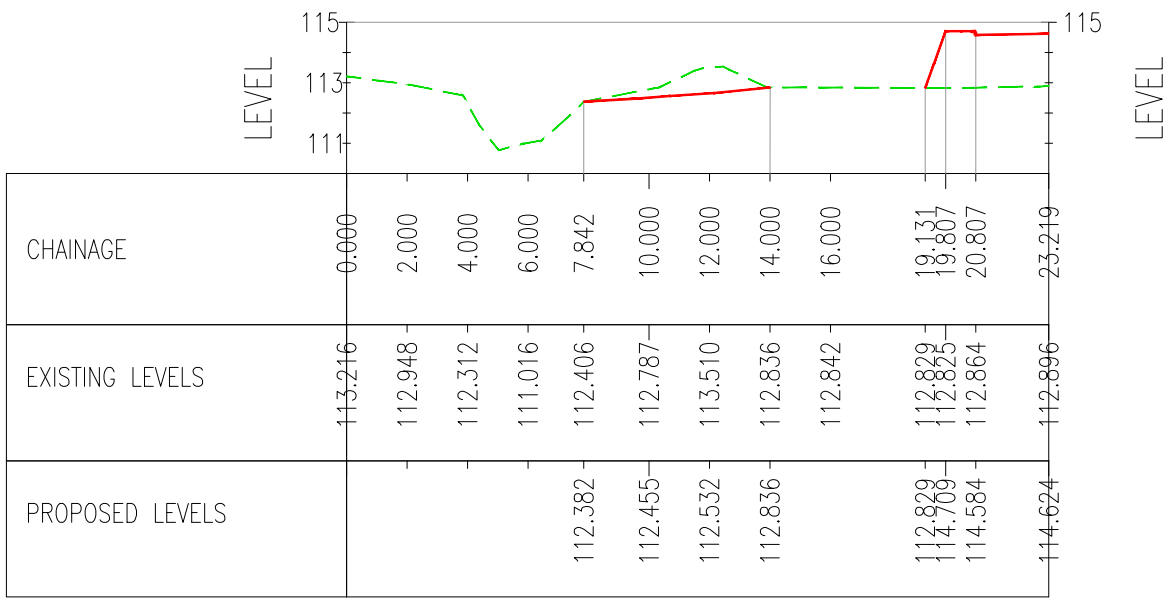
SECTION M-M
