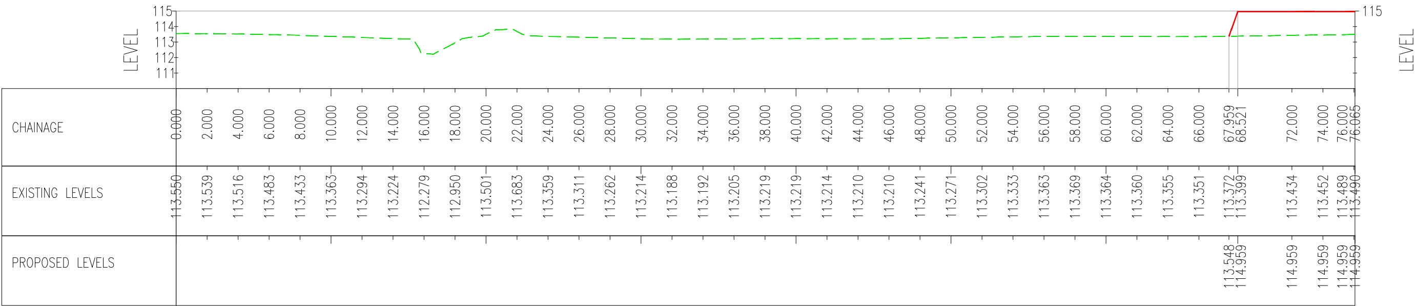
SECTION O-O
