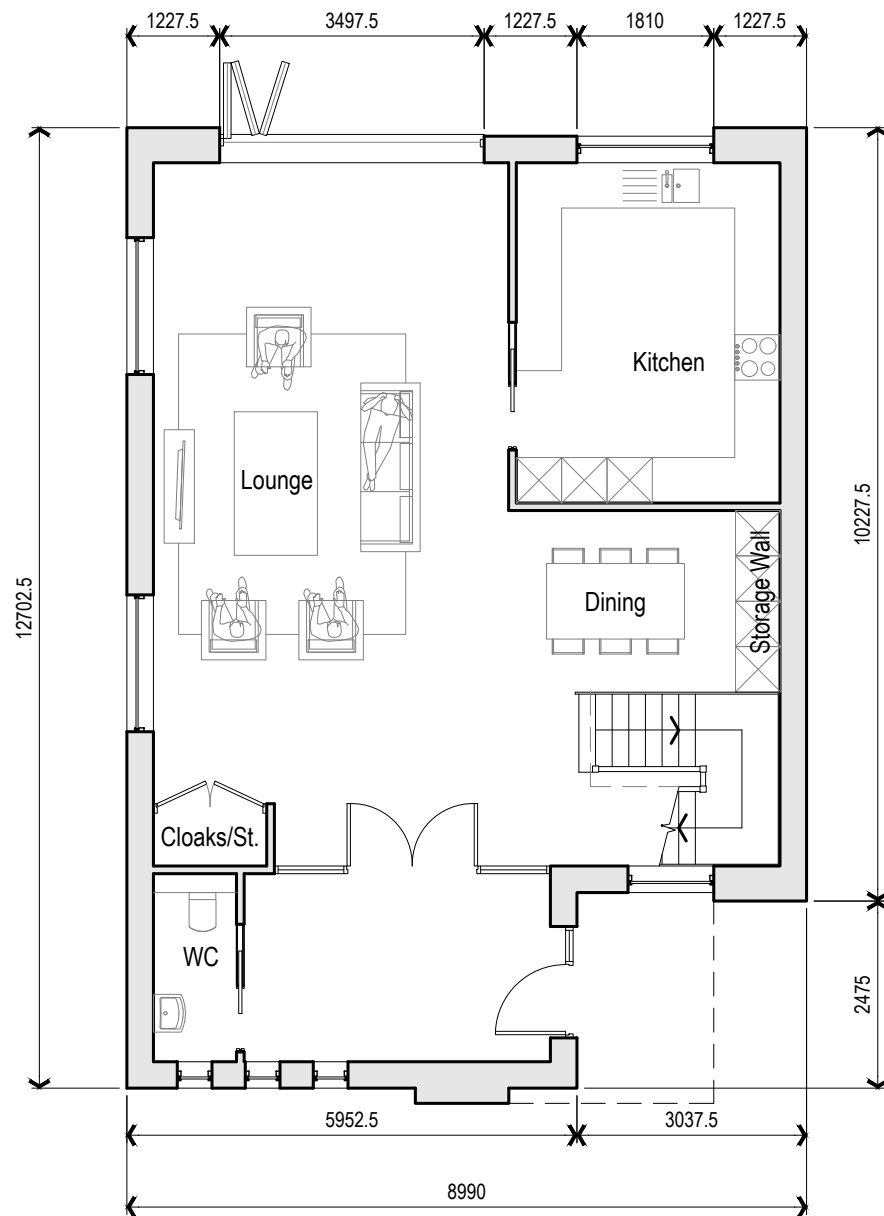
PROPOSED GROUND FLOOR PLAN 1:100@A3
