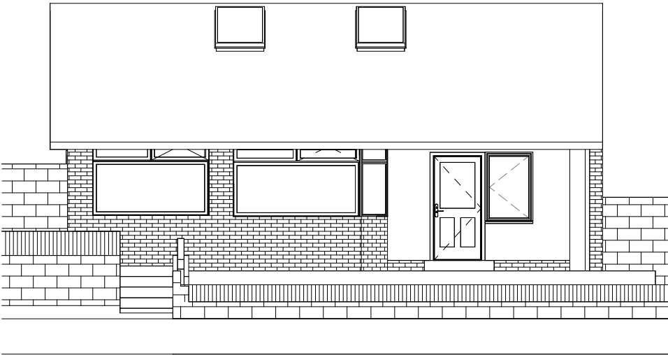
1 Proposed Front Elevation 1 : 100
