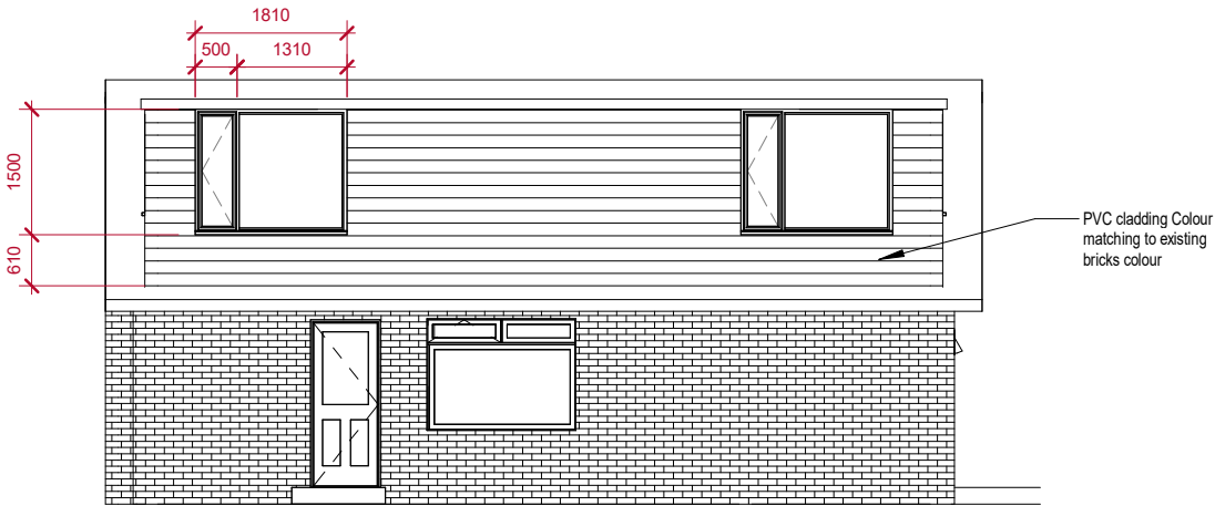
1 Proposed Front Elevation 1 : 100
