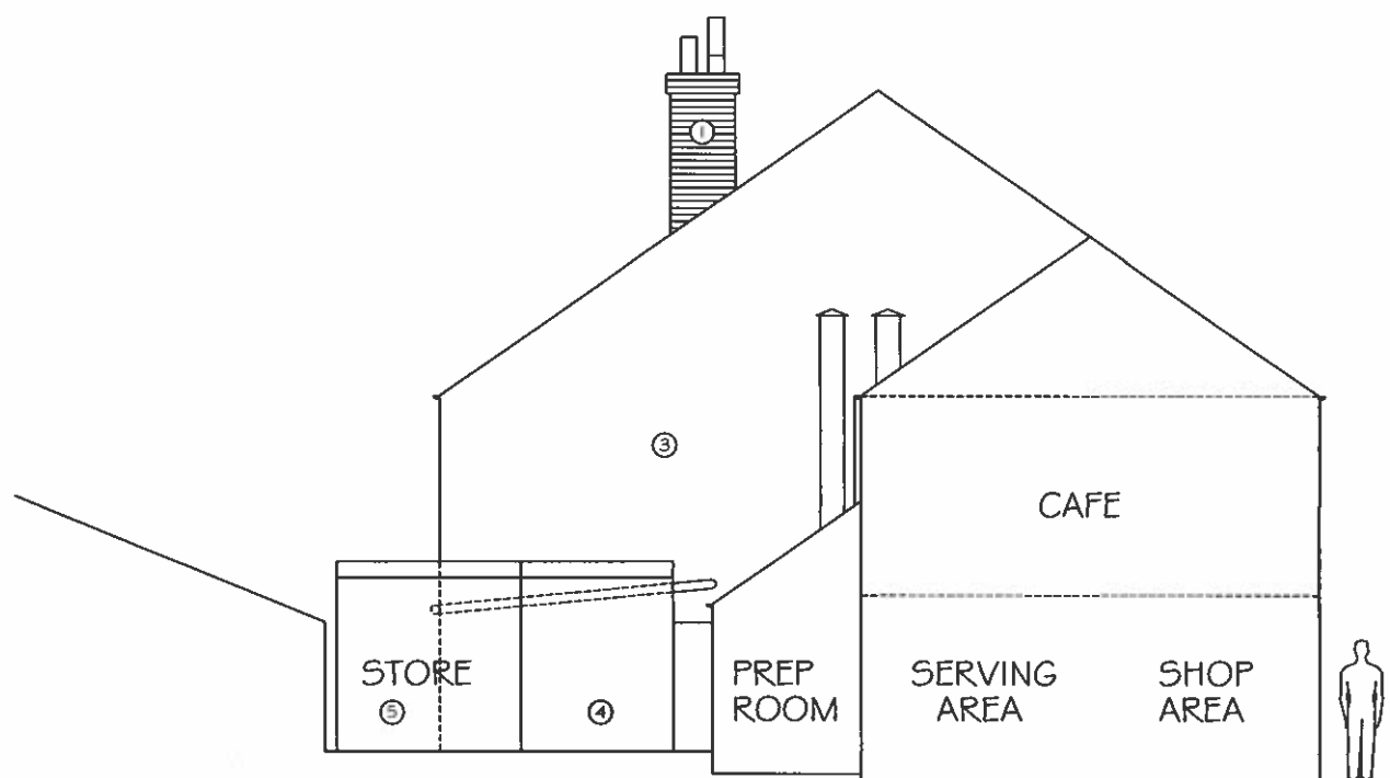
EXISTING ELEVATION [LOOKING TOWARDS NO. 88/88A] 1:100
