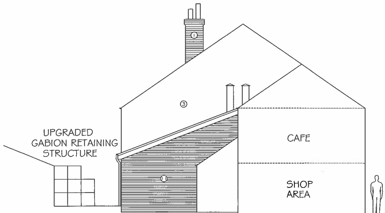
PROPOSED ELEVATION [LOOKING TOWARDS NO. 88/88A] 1:100
