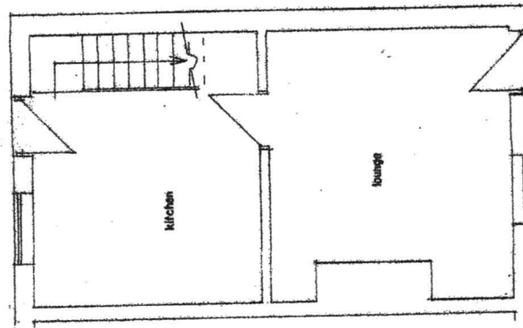
G.F. PLAN (EXISTING)
