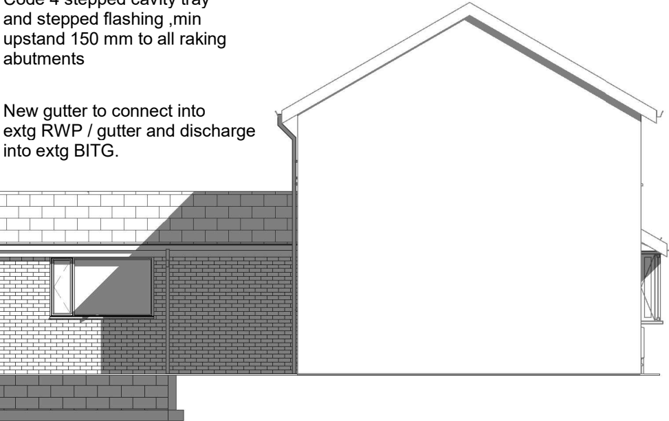
4 Neighbouring Elevation 1 : 100
