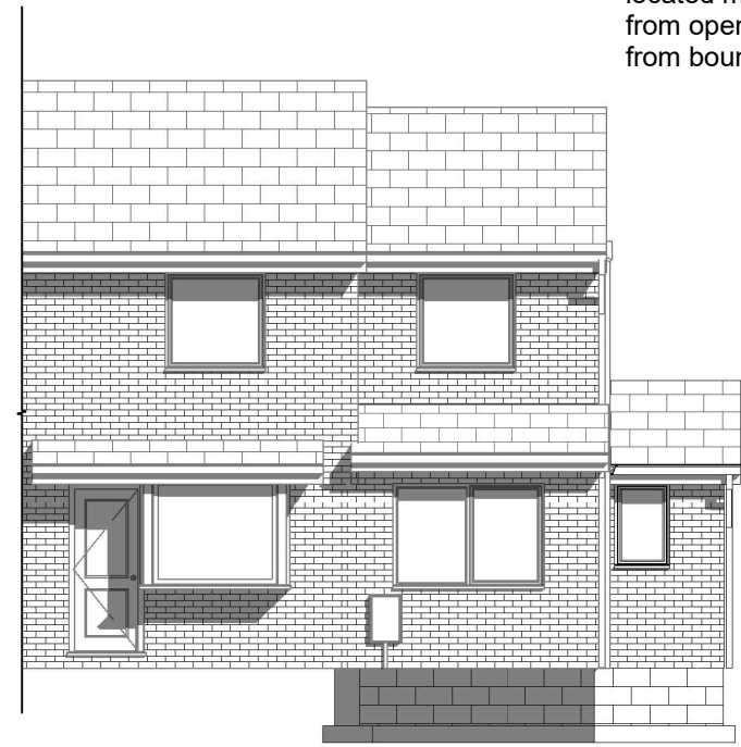
1 Front Elevation 1 : 100
