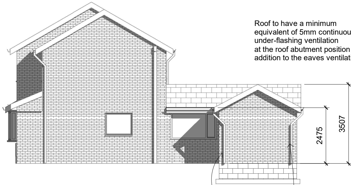
2 Gable Elevation 1 : 100
