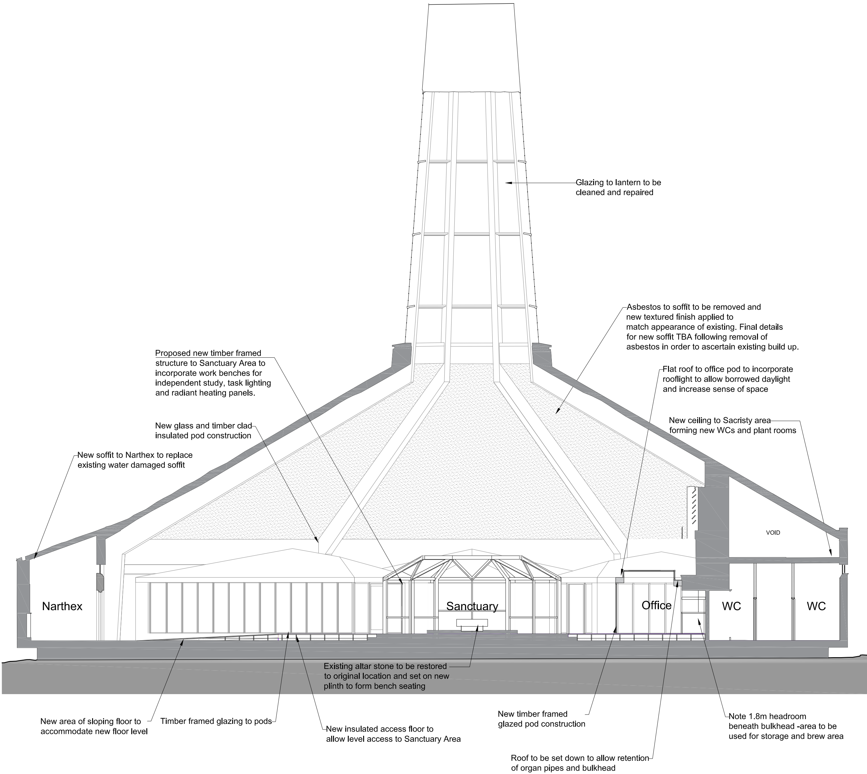
Proposed Section A
