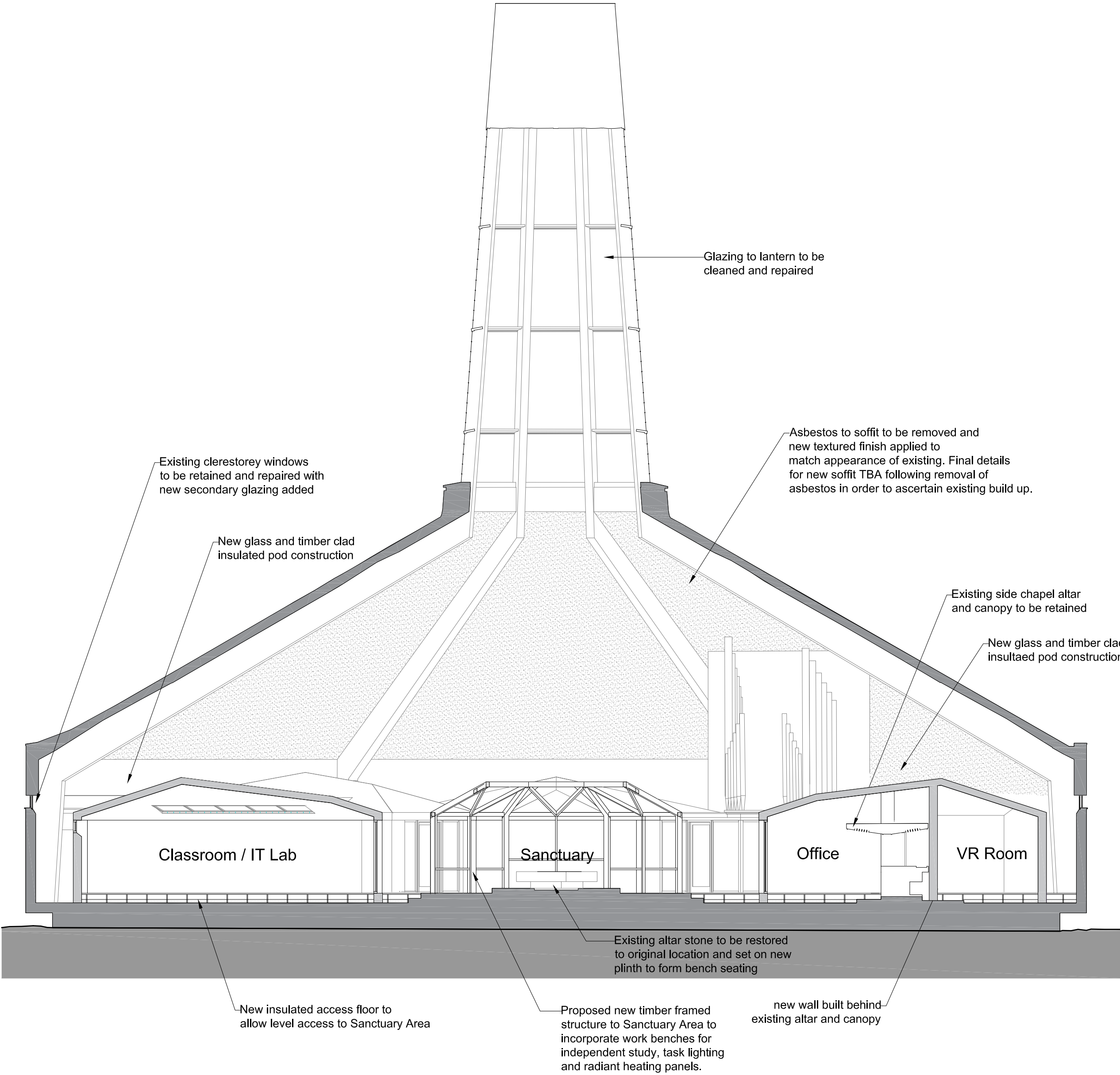
Proposed Section B
