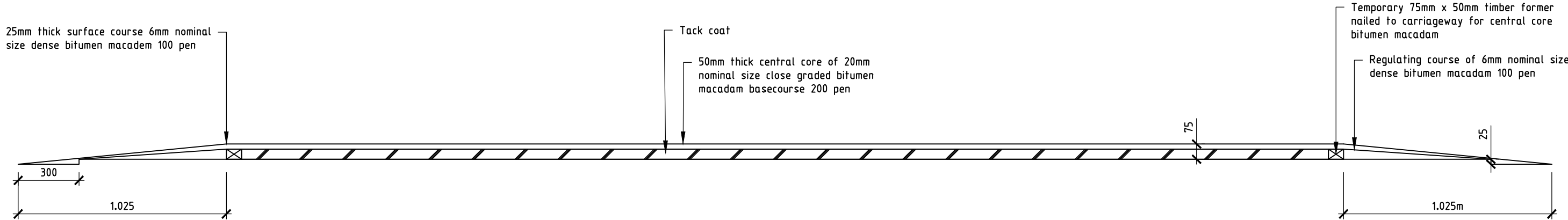
ROAD HUMPH CONSTRUCTION DETAIL SCALE 1:20
