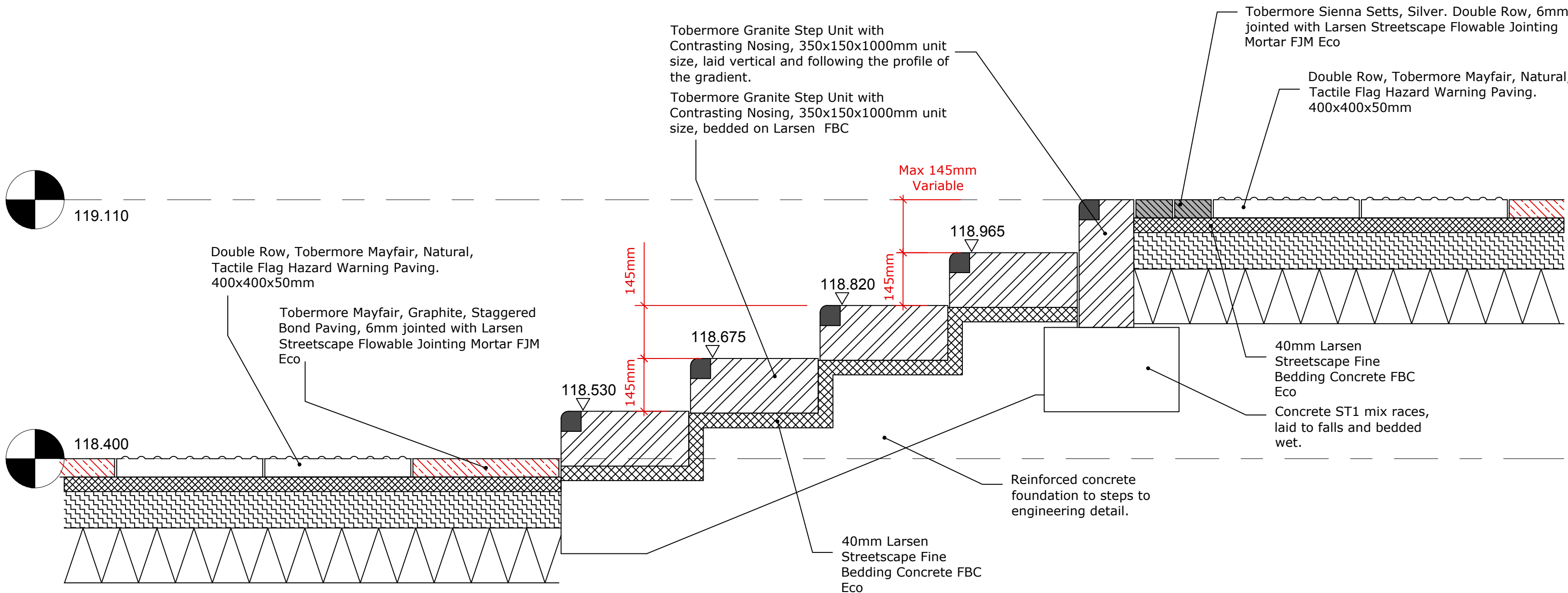
Section Through Steps 1:10
