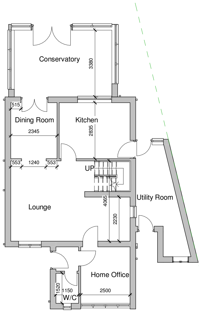
Existing Groundfloor 1 : 100
