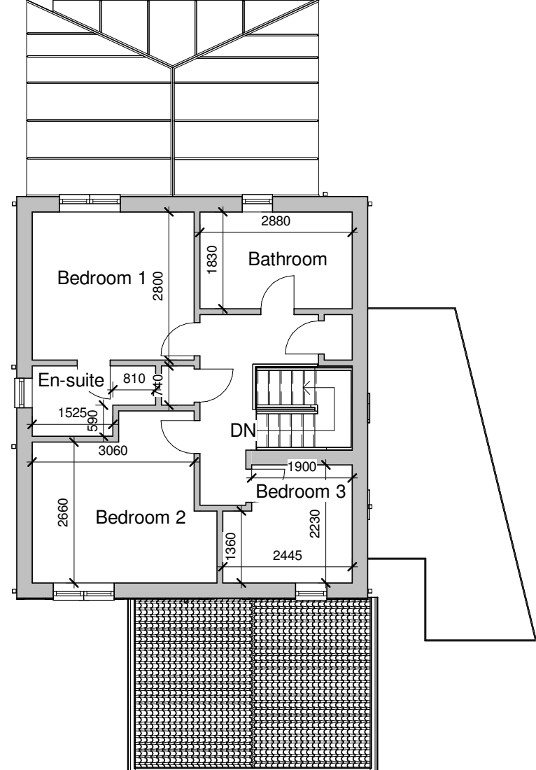
Existing Firstfloor 1 : 100
