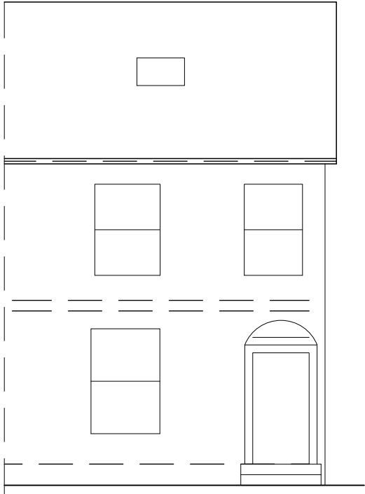
FRONT ELEVATION (EXISTING & PROPOSED)
