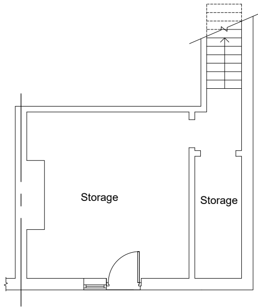
BASEMENT (EXISTING)
