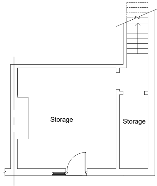
BASEMENT (PROPOSED)
