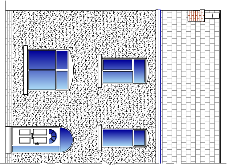
Proposed Front Elevation 1:100
