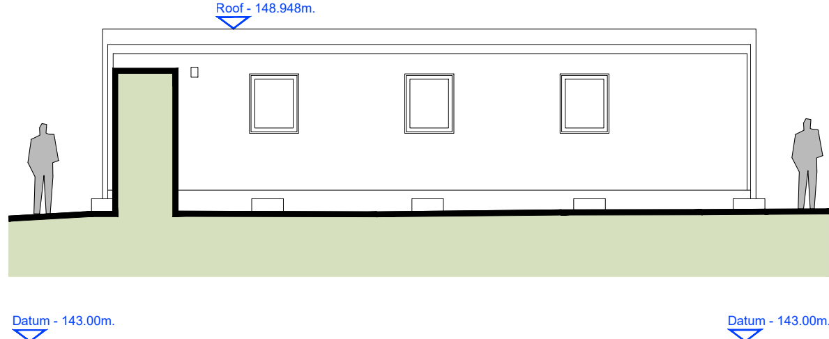
EXISTING ELEVATION 8 (BUILDING 4) 1:100@A1
