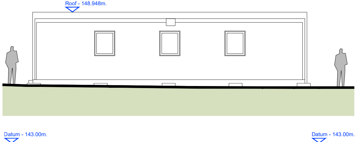
EXISTING ELEVATION 6 (BUILDING 4) 1:100@A1
