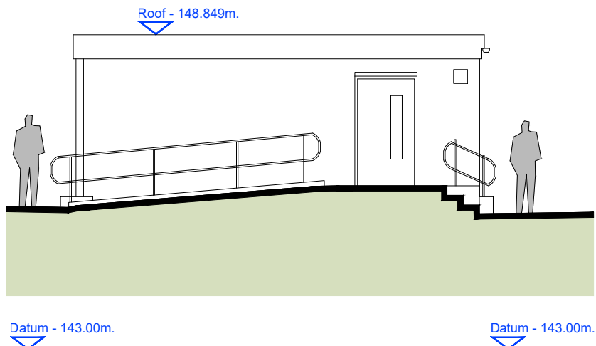
EXISTING ELEVATION 2 (BUILDING 5) 1:100@A1
