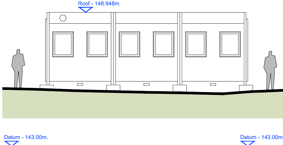
EXISTING ELEVATION 7 (BUILDING 4) 1:100@A1
