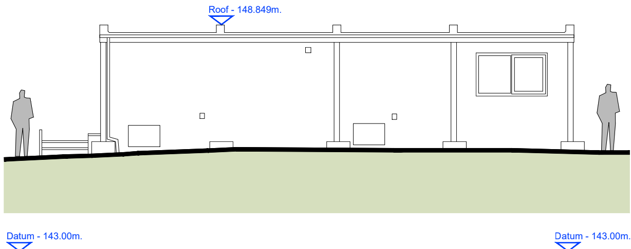
EXISTING ELEVATION 3 (BUILDING 5) 1:100@A1
