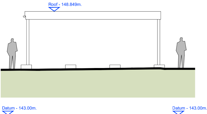
EXISTING ELEVATION 4 (BUILDING 5) 1:100@A1
