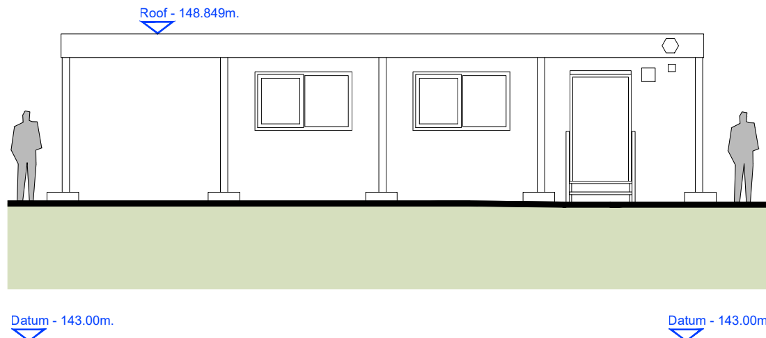
EXISTING ELEVATION 1 (BUILDING 5) 1:100@A1
