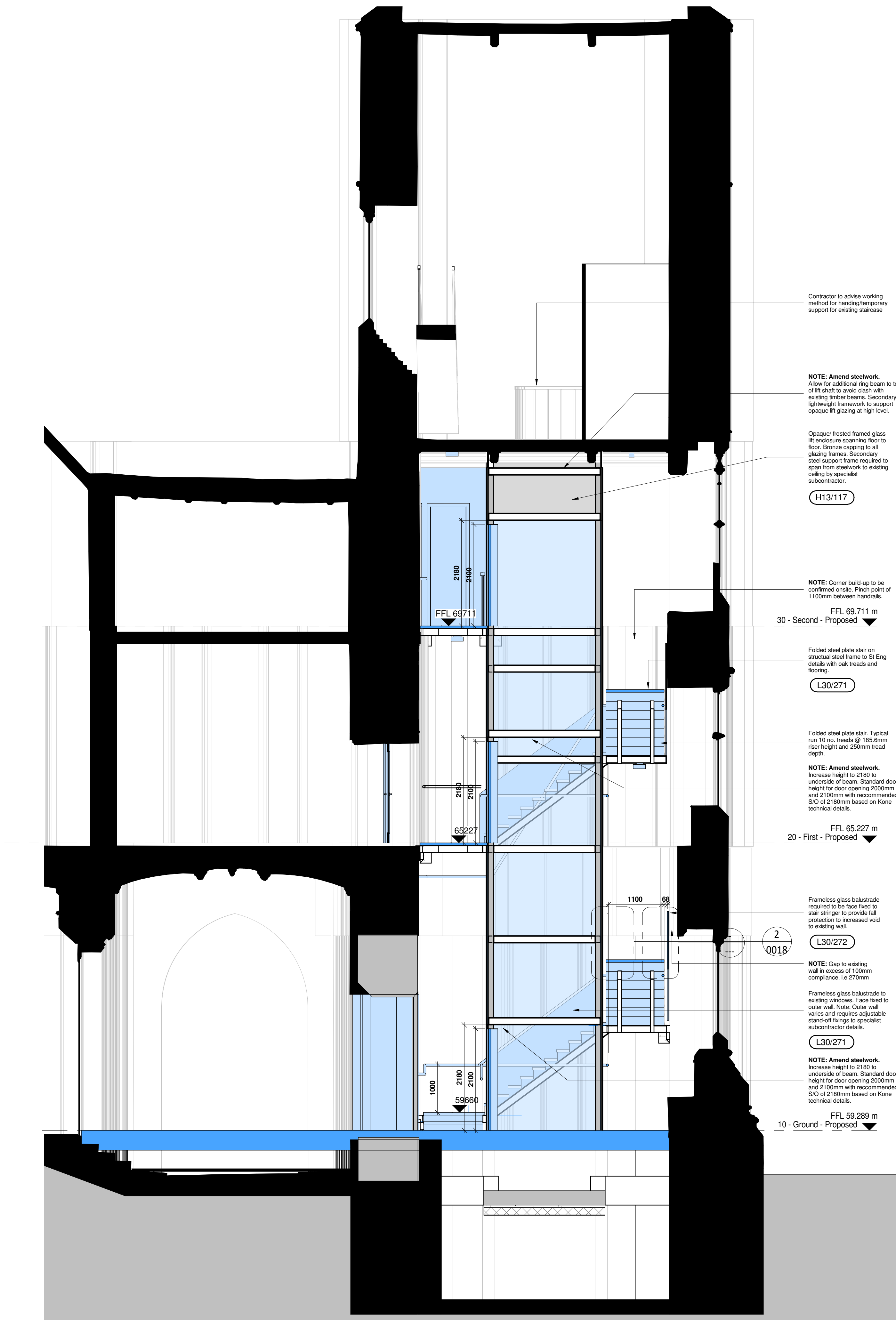
2D View 1 : 50
