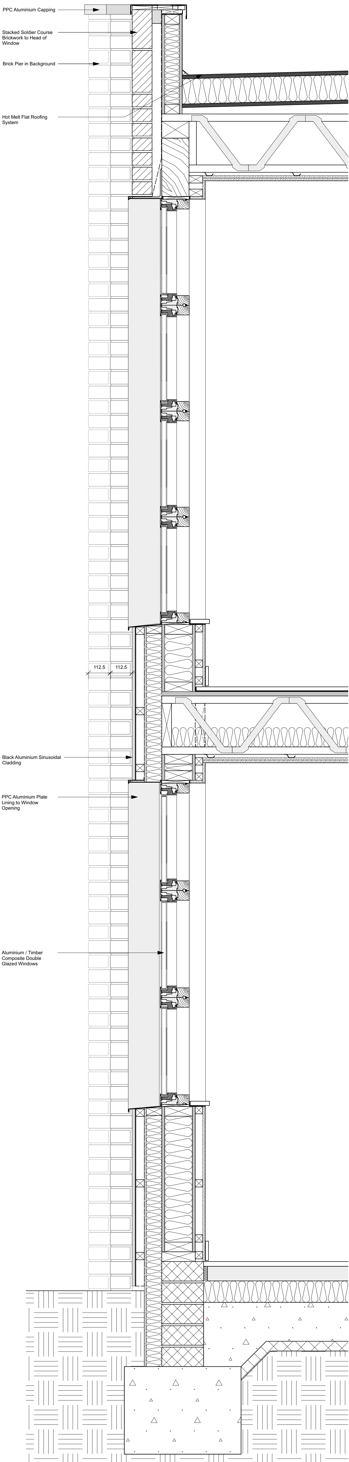
1 Proposed Section AA Scale: 1:10
