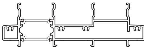
PUR201200 Outerframe Track
