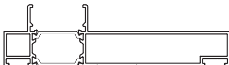
PUR203202 Outerframe Jamb
