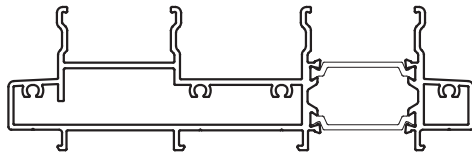
PUR200201 Outerframe Track
