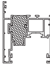
PUR206207 Door Stile
