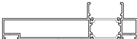
PUR202203 Outerframe Jamb
