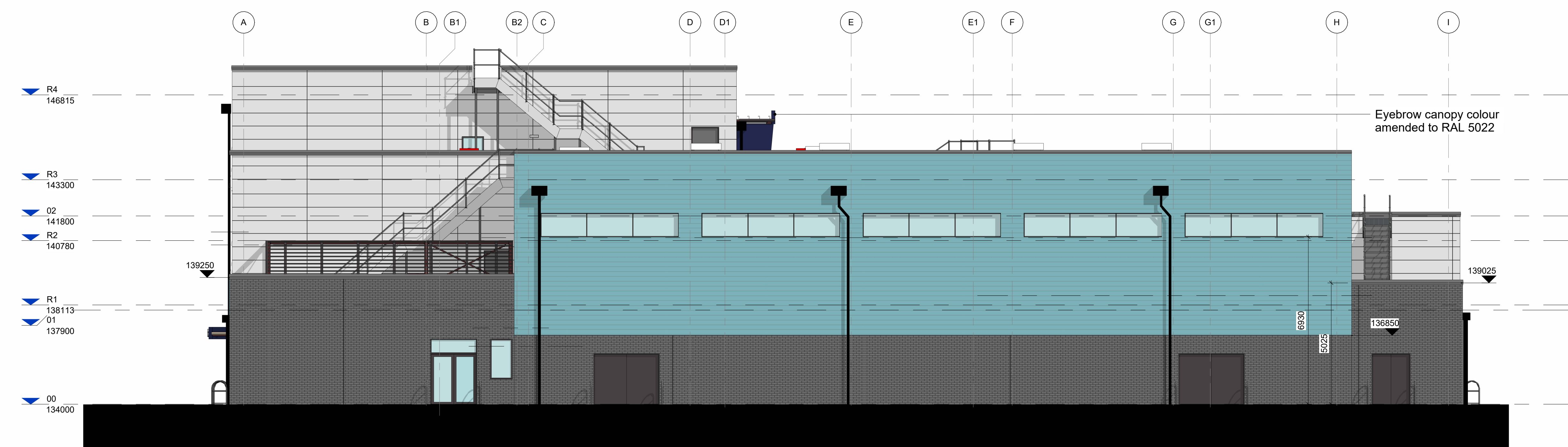
West Elevation 1 : 100
