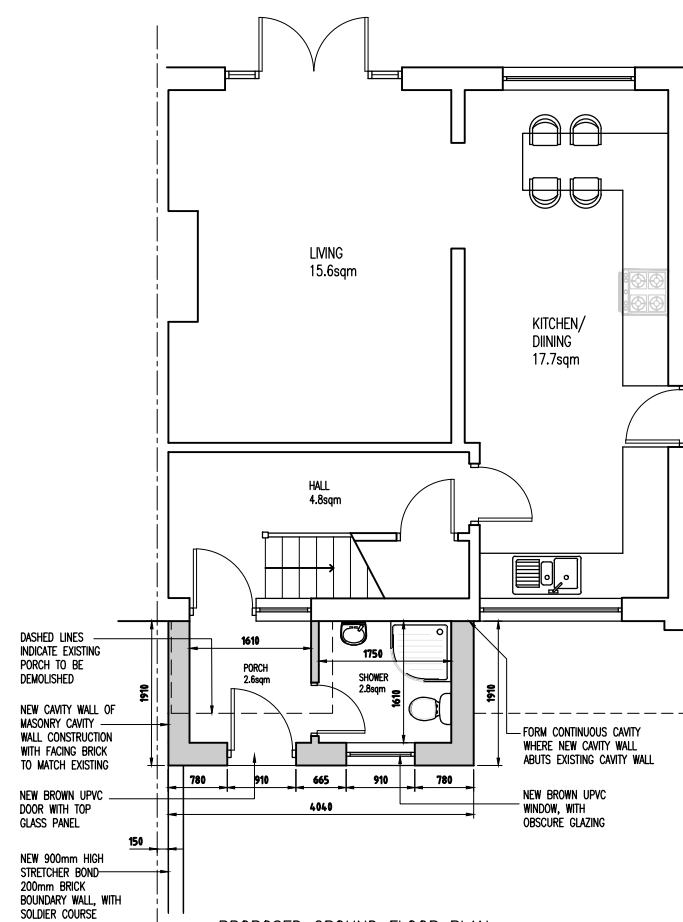
PROPOSED GROUND FLOOR PLAN 1:100 @ A3
