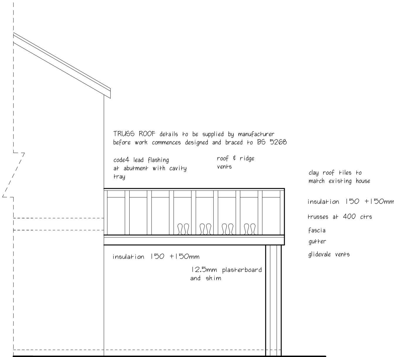
Proposed side elevation (East) cross section scale:1:50
