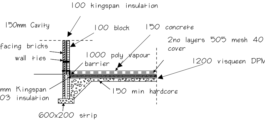
FOUNDATION DETAIL
