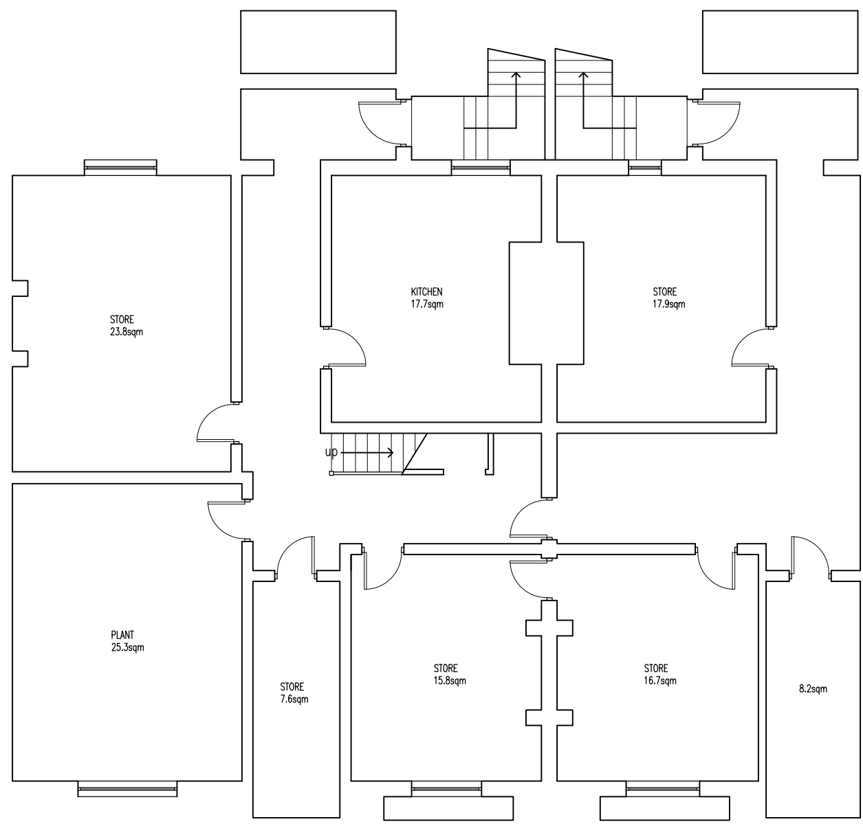
PROPOSED BASEMENT FLOOR PLAN 1:100 @ A3
