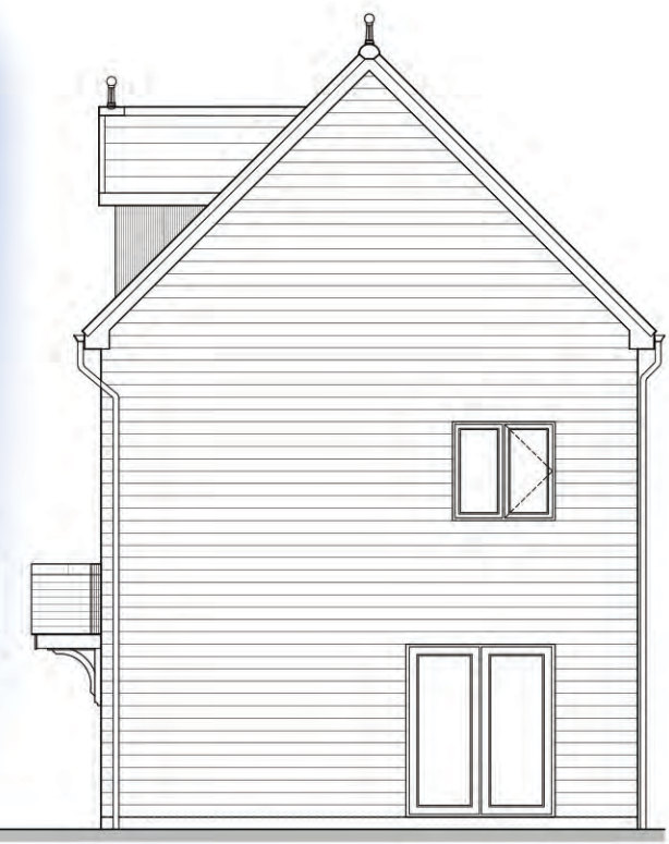
Rear Elevation
