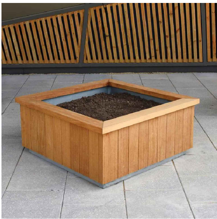
Proposed Swindon Planter Timber Planter With Galvanized Frame 990mm x 990mm x 450mm
