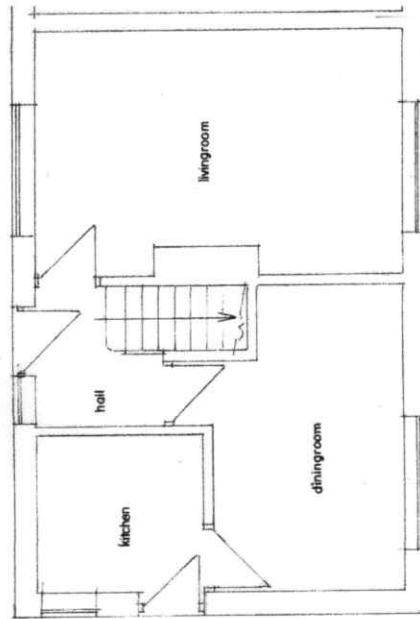
G.F. PLAN (EXISTING)
