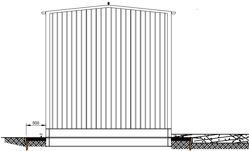
ELEVATION B UKPN SUBSTATION ACCESS
