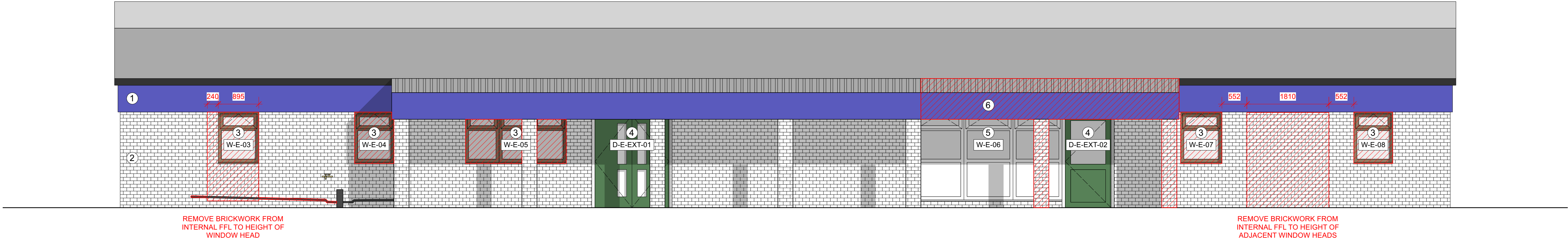
1 Existing North West Elevation Scale: 1:50
