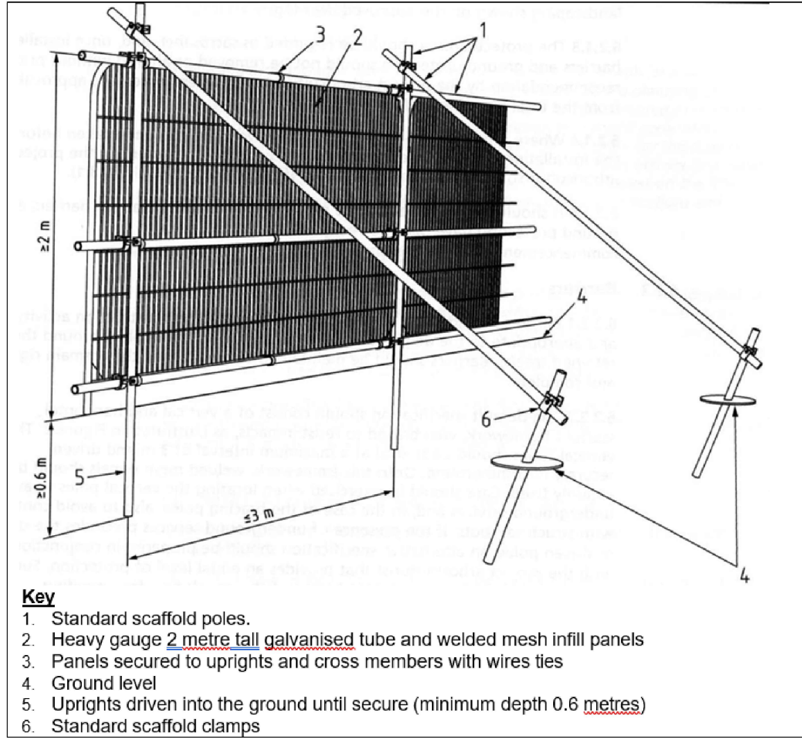
Figure 2: BS5837:2012 Default specification for protective barrier
