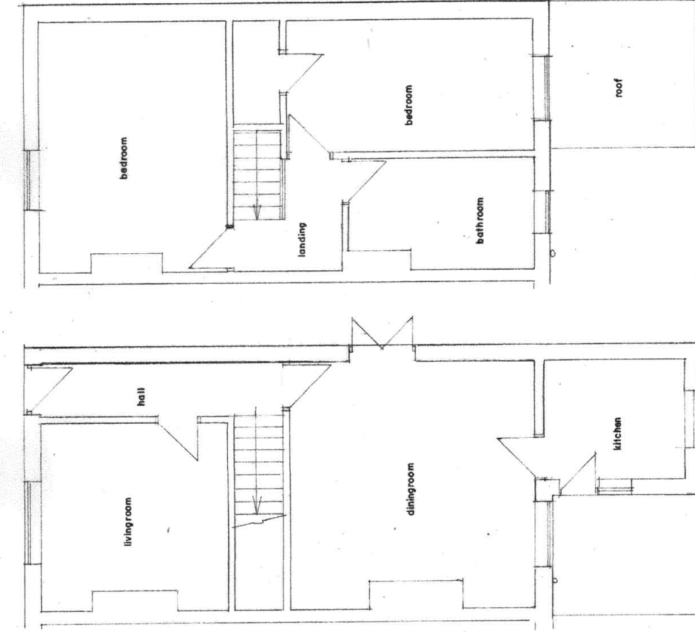
G.F. PLAN (EXISTING)
