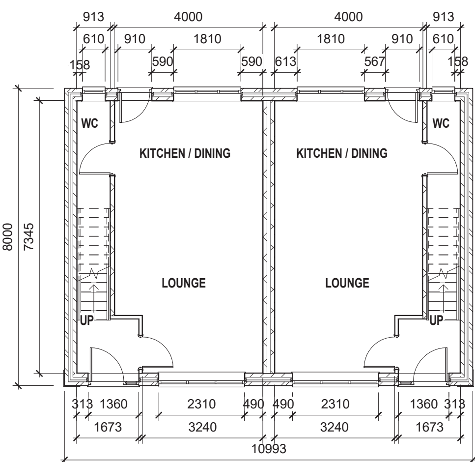
1 GROUND FLOOR PLAN 1 : 100
