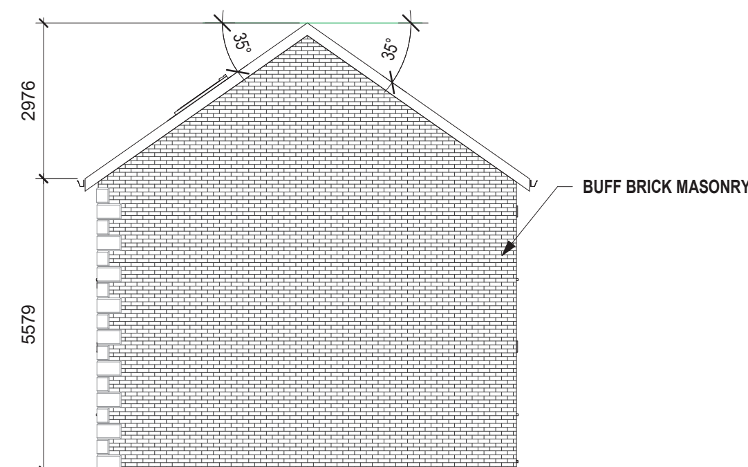
6 GABLE ELEVATION 1 : 100
