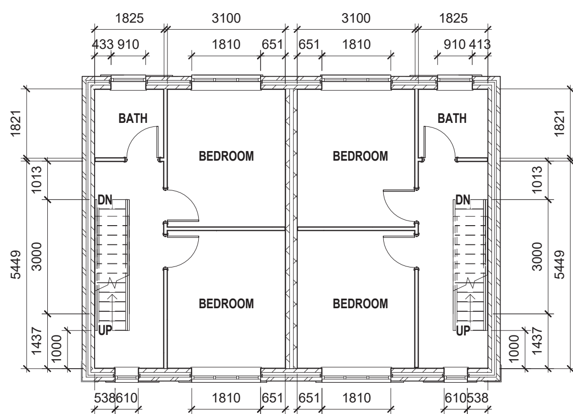
2 FIRST FLOOR PLAN 1 : 100
