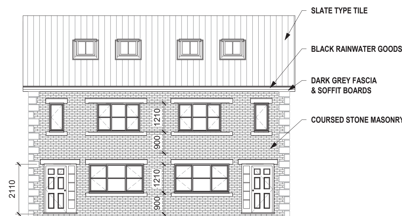
5 FRONT ELEVATION 1 : 100
