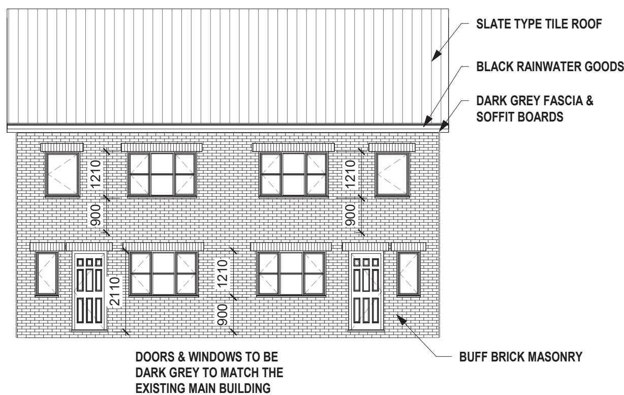
8 REAR ELEVATION 1 : 100
