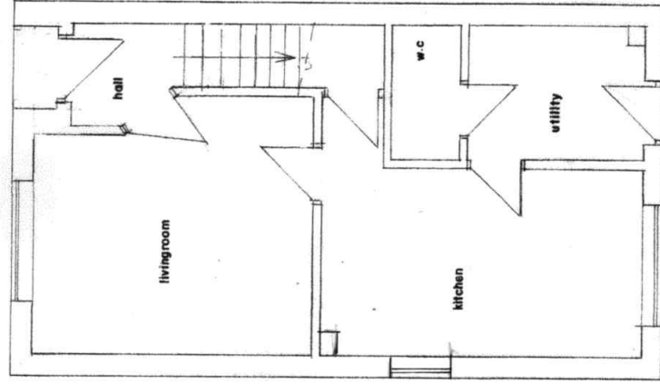
G F PLAN (EXISTING)
