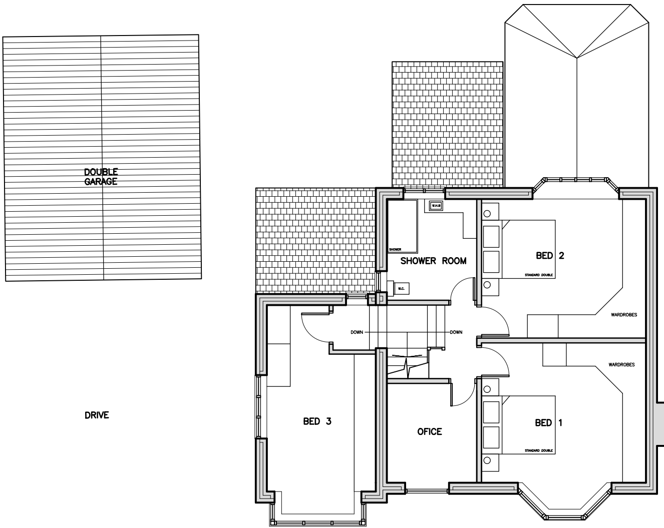
EXISTING FIRST FLOOR LEVEL
