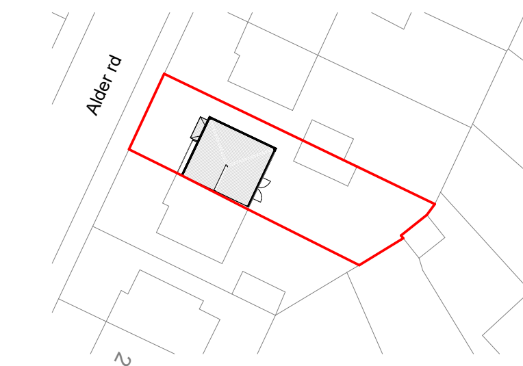
2 Existing Block Plan 1 : 500
