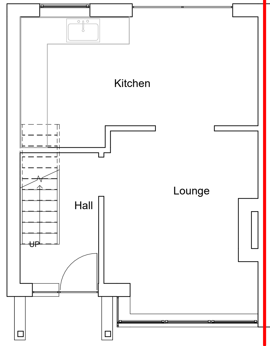
3 Existing Ground Floor 1 : 50
