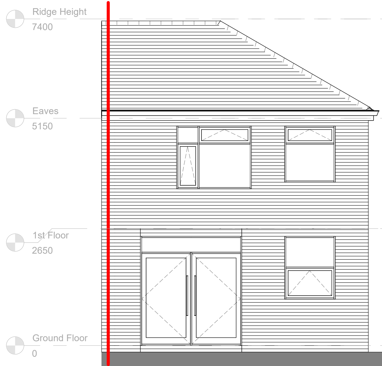
4 Existing Rear Elevation 1 : 50
