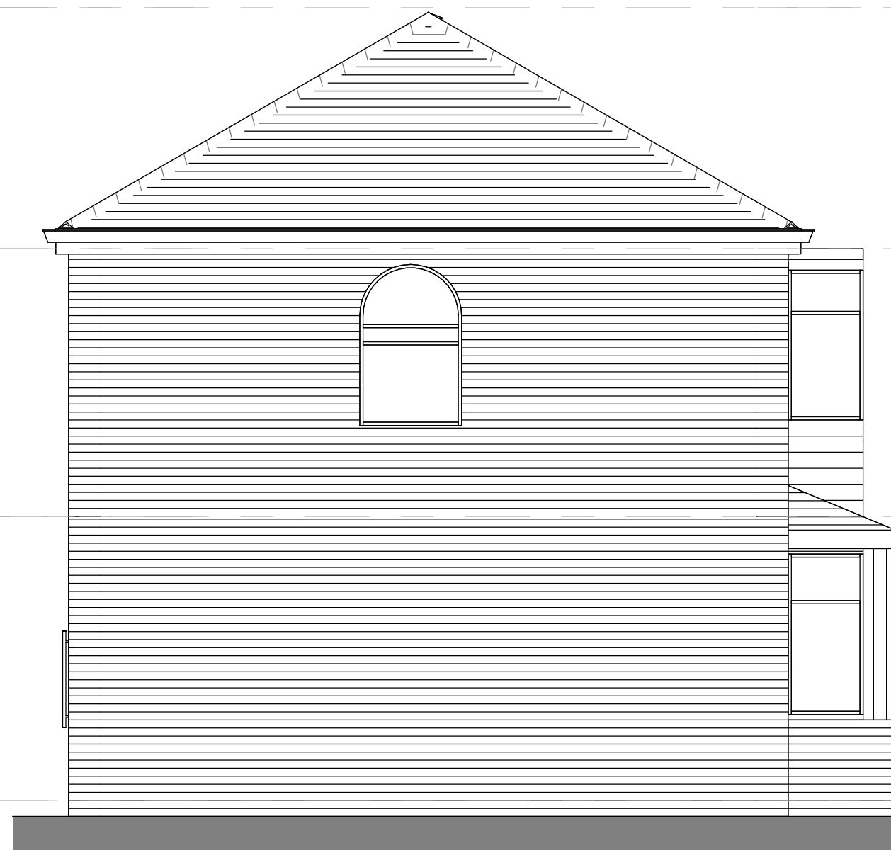
7 Existing LHS Elevation 1 : 50
