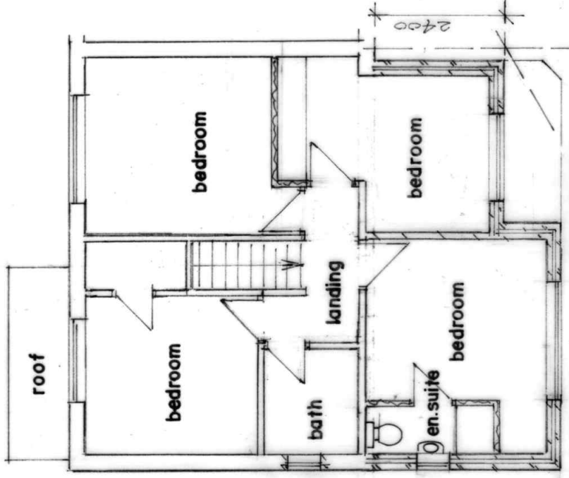
FIRST FLOOR PLAN (PROPOSED)
