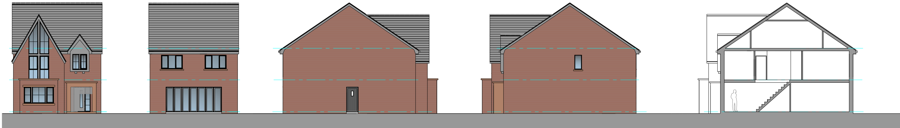
Front Elevation
