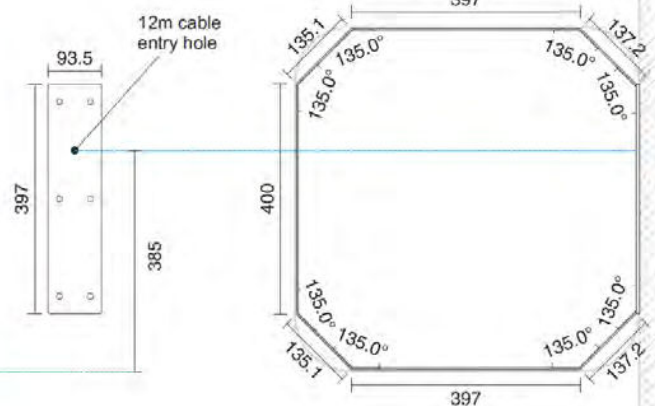
LED layout
