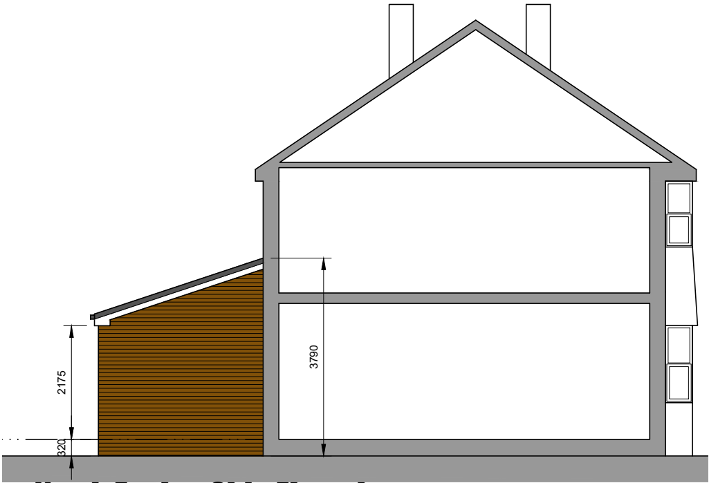
North Facing Side Elevation
