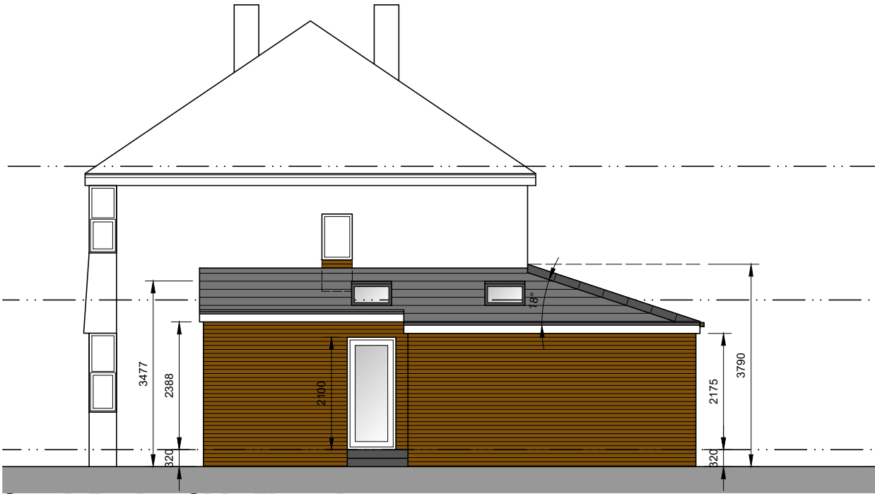
South Facing Side Elevation
