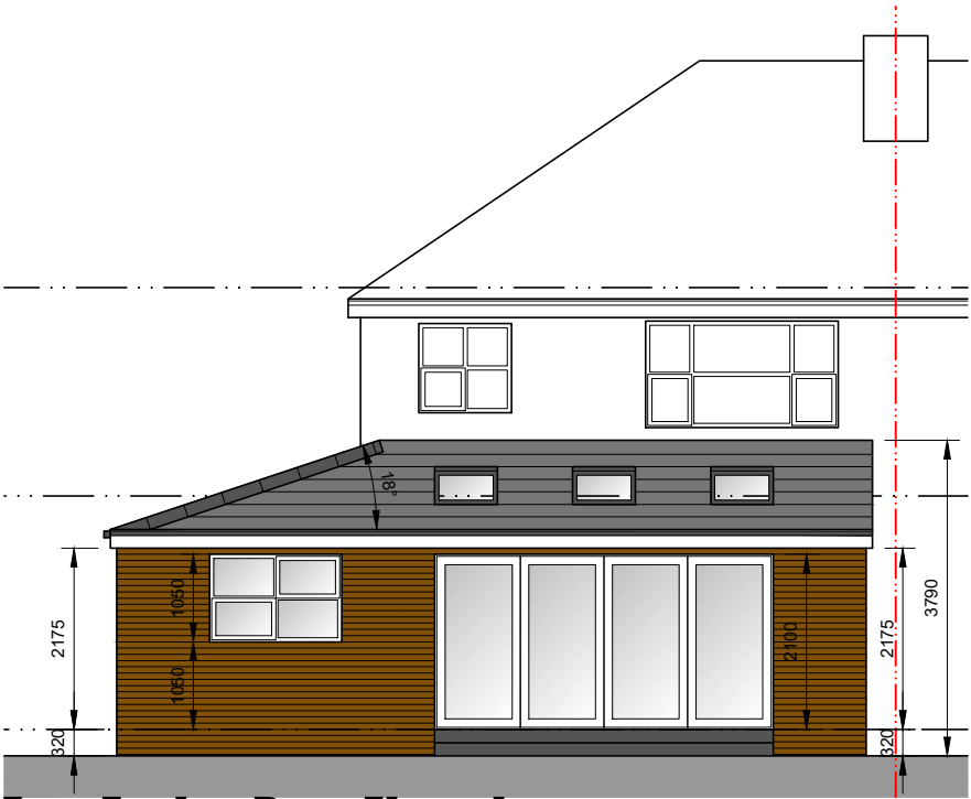
East Facing Rear Elevation
