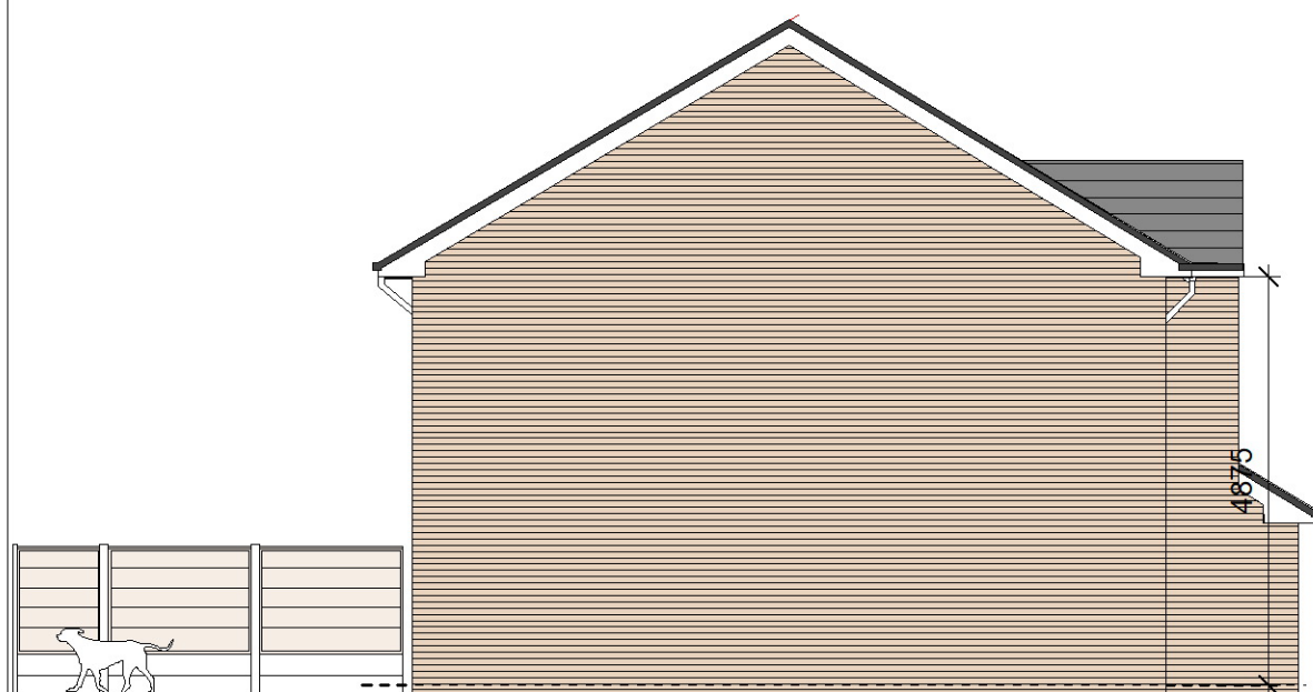
SIDE ELEVATION AS EXISTING/PROPOSED (NORTH)
