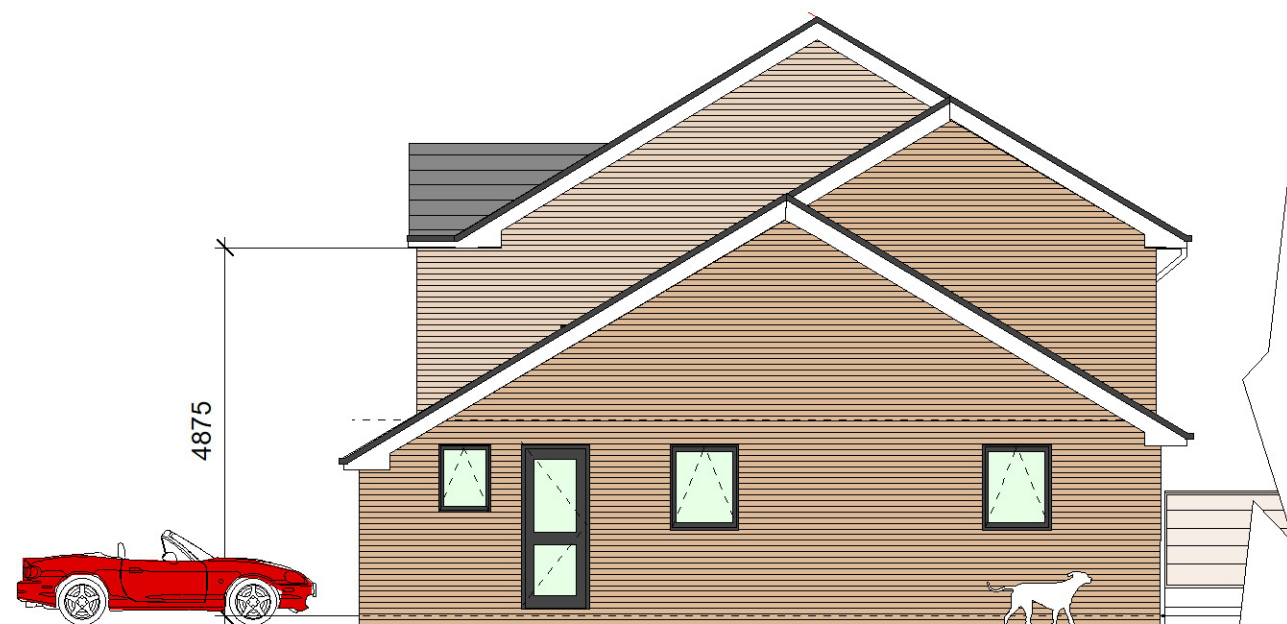
SIDE ELEVATION AS PROPOSED (SOUTH)
