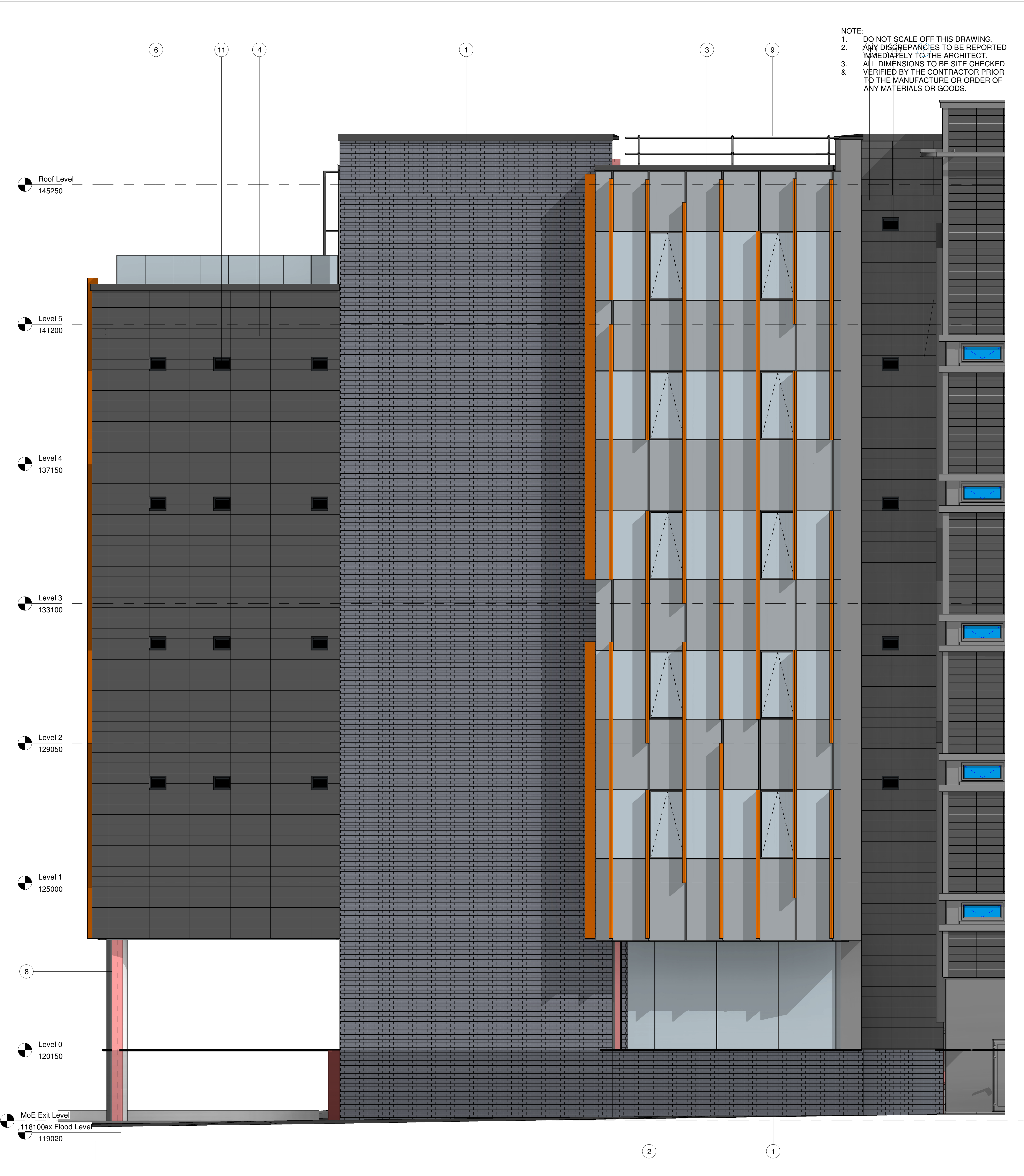
Detailed GA Elevation - South West 1 to 50 1 : 50
