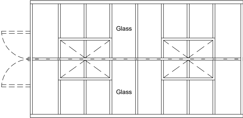
Roof Plan
