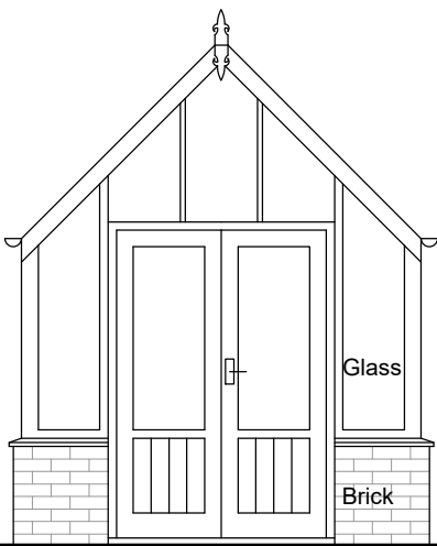
Front Elevation (south-east)
