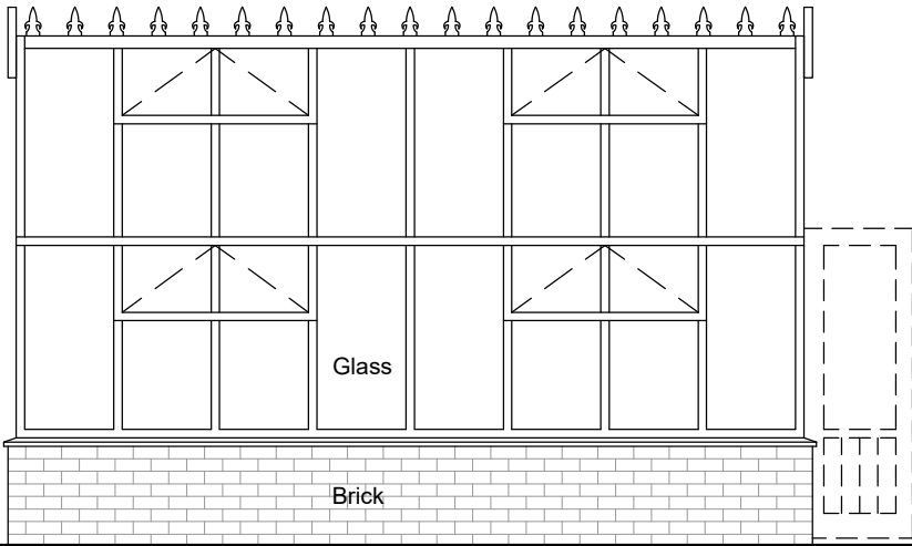
Side Elevation (south-west)
