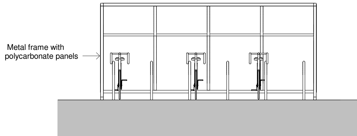
3 Proposed Front Elevation _Bike Store 1 : 50
