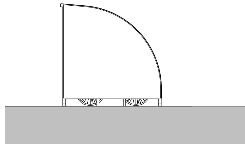
6 Proposed Side Elevation _Bike Store 1 : 50
