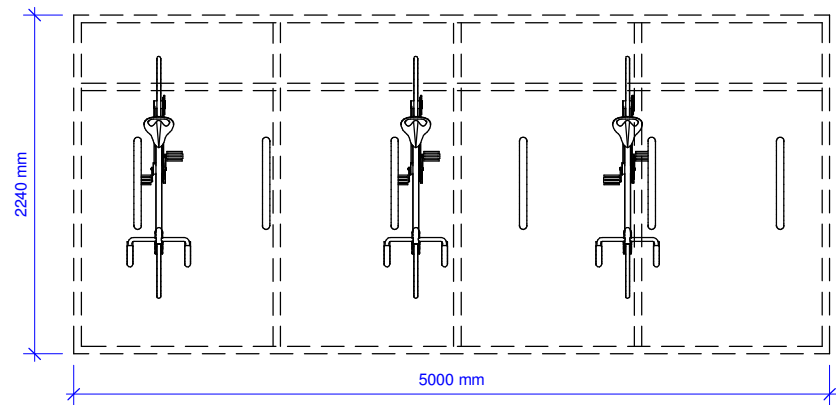
1 Proposed Floor Plan _Bike Store 1 : 50
