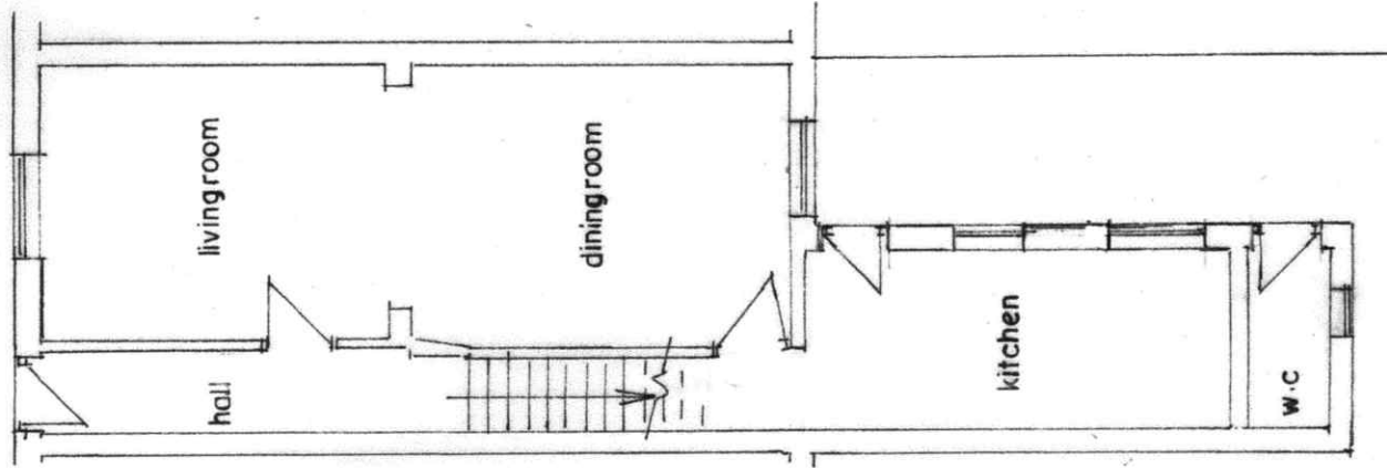
G.F. PLAN (EXISTING)
