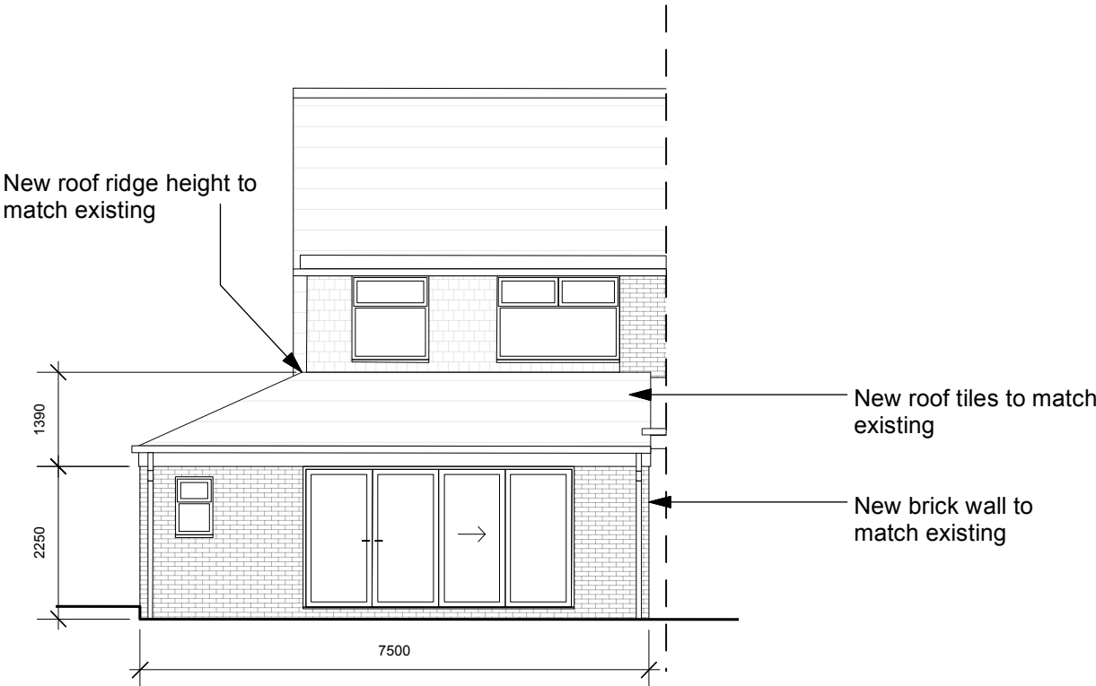
SOUTH (REAR) ELEVATION
