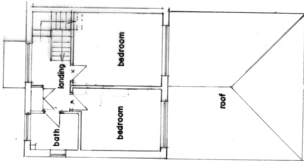
FIRST FLOOR PLAN (PROPOSED)
