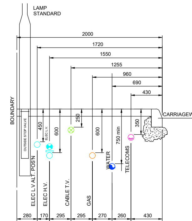
DETAIL 'B' NATIONAL JOINT UTILITIES GROUP (IN LUG) POSITIONING OF UTILITIES MAINS IN 2m FOOTWAY
