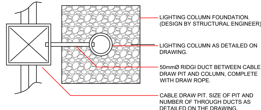
EXTERNAL LIGHTING COLUMN CABLE PIT DETAIL
