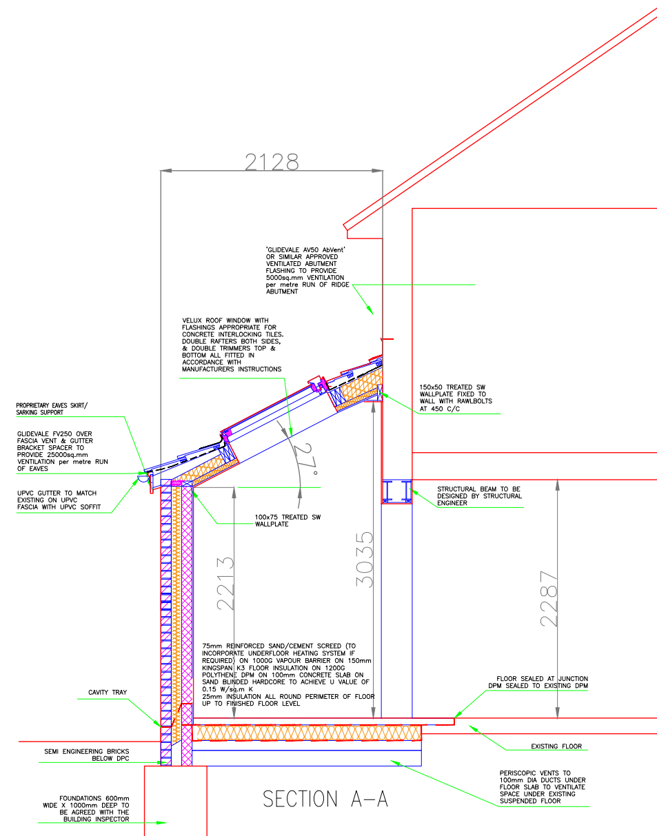
Proposed Section @1:50
